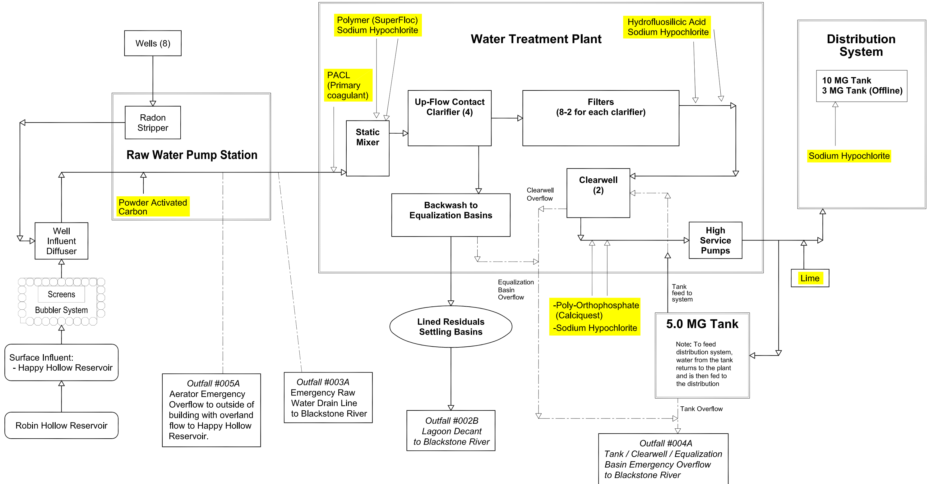
PWSB - PROCESS FLOW DIAGRAM
